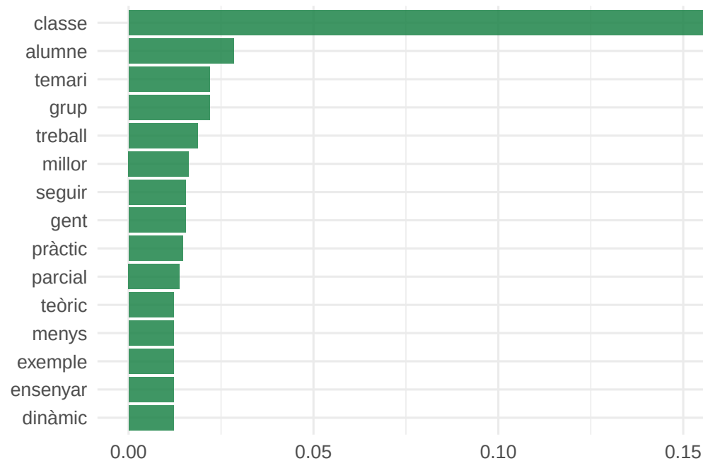
Topic 3
