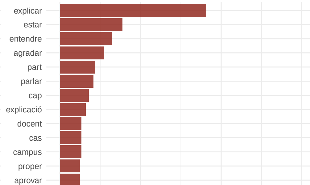
Topic 2
