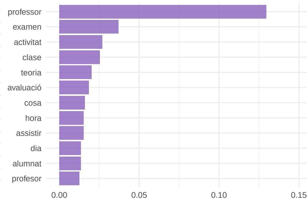
Topic 4
