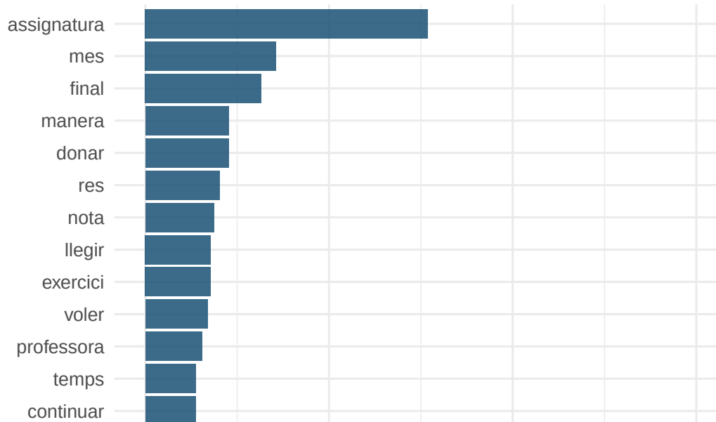
Topic 1
